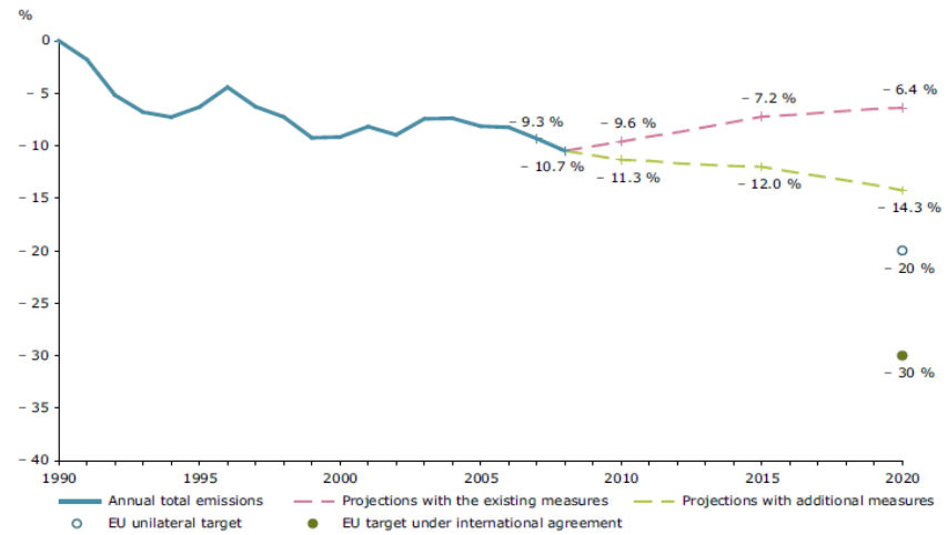
Figure ES.4 EU-27 GHG emission trends and projections to 2020
