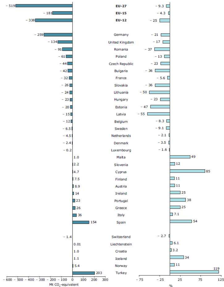
Figure 2.7 Changes in greenhouse gas emissions in Europe, 1990–2007
